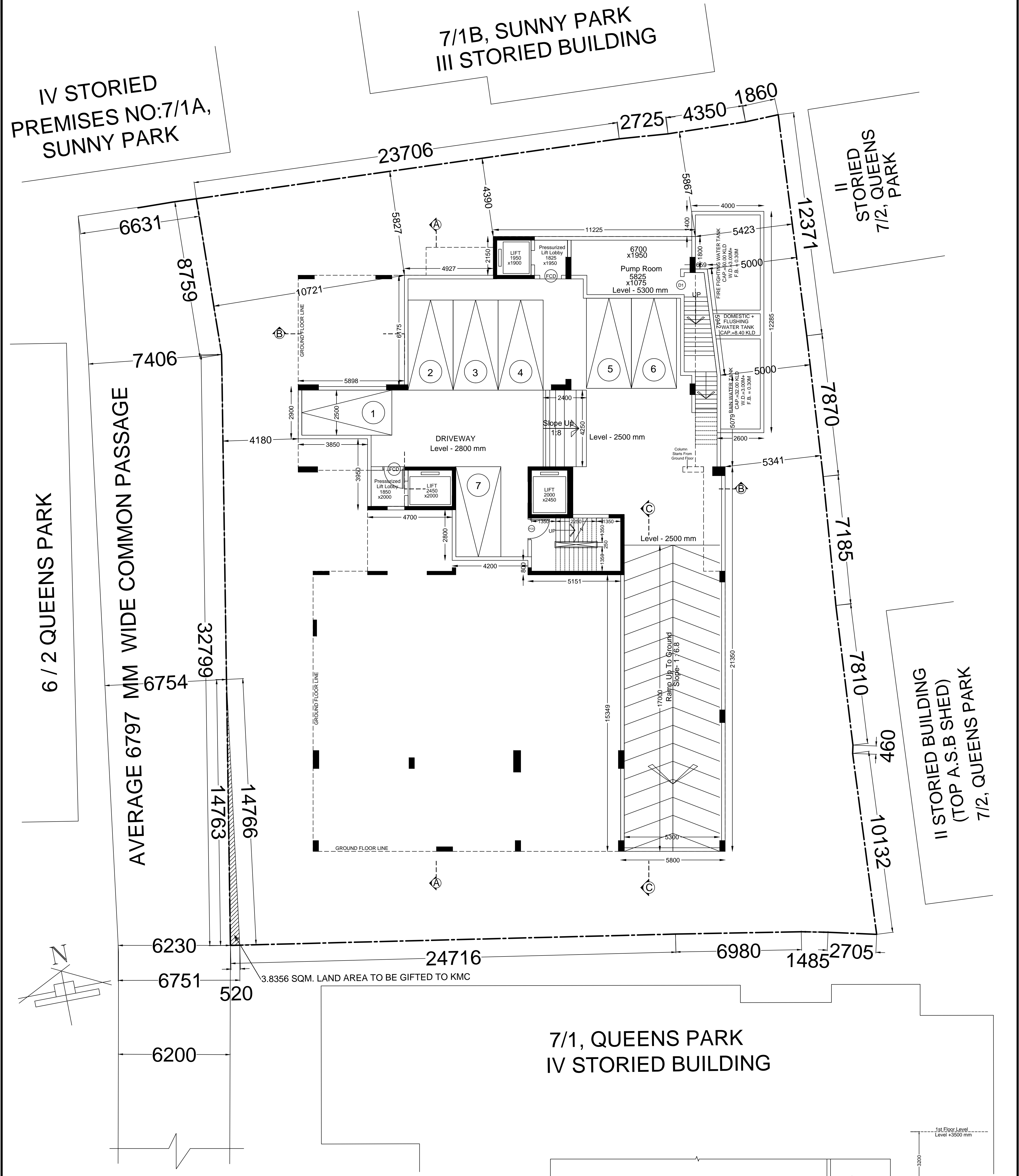
BASEMENT PLAN SCALE - 1:100
